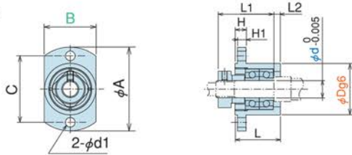
Round type fixed side Support unit
