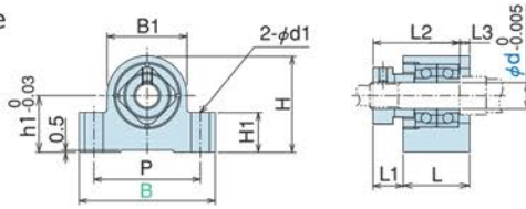
Square type fixed side Support unit
